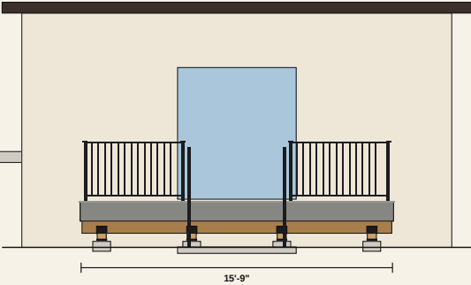
FRONT ELEVATION — from the yard
